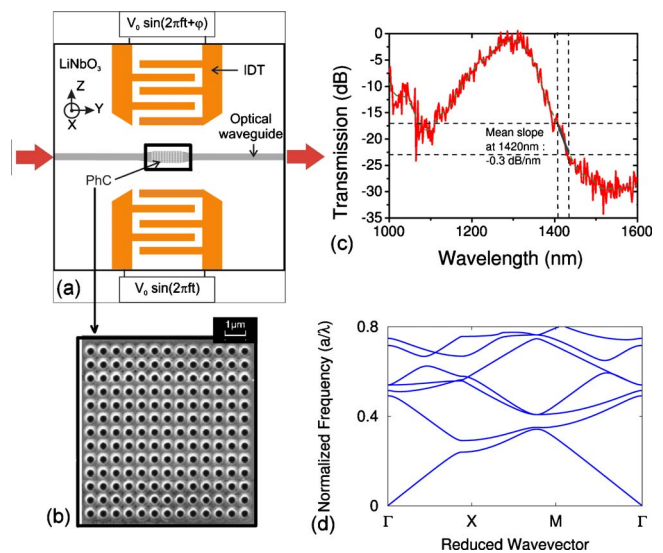
FIG. 1. (Color online) (a) Schematics of the acousto-optic modulators. (b) Scanning electron microscope image of the fabricated square lattice air/LiNbO 3 PhC. Pitch a=825 nm, diameter d=412 nm. (c) Measured optical transmission through the PhC (solid red line). Results obtained by normalizing the optical intensity transmitted through the nanostructured waveguide with the intensity through a single waveguide realized in the same conditions without any PhC. The dashed green line is the experimental result filtered using a low pass filter. (d) Corresponding band structure.
