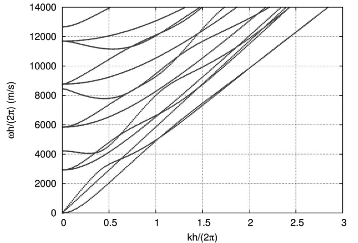
Fig. 2. Band structure computed by the PWE method for the single elastic plate of Fig. 1. The considered material is (100) silicon. Thirty-one harmonics are used and a/h = 1.5 .
