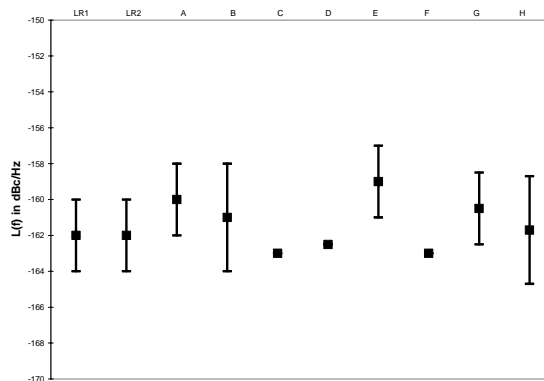
Figure 5: SSB phase noise at 100 kHz from the 100 MHz carrier. Uncertainties given at 2\sigma
