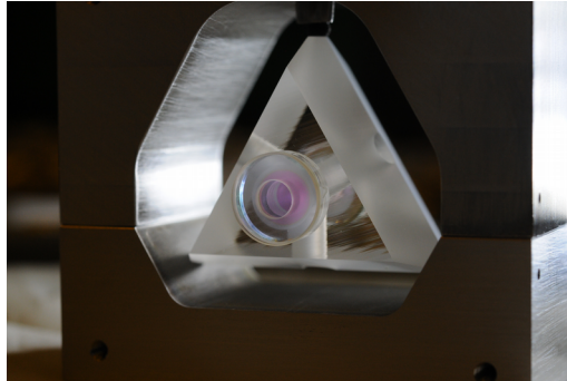
Compact ULE cavity in its stainless steel spacer.
